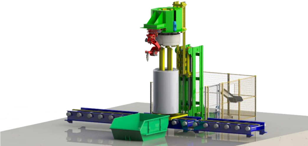
Figure 8. Illustration of TRIMBOT station in vertical configuration.
