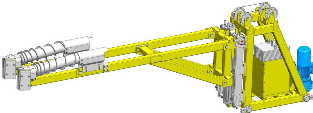
Figure 4. Illustration of the Internal ring transfer trolley
